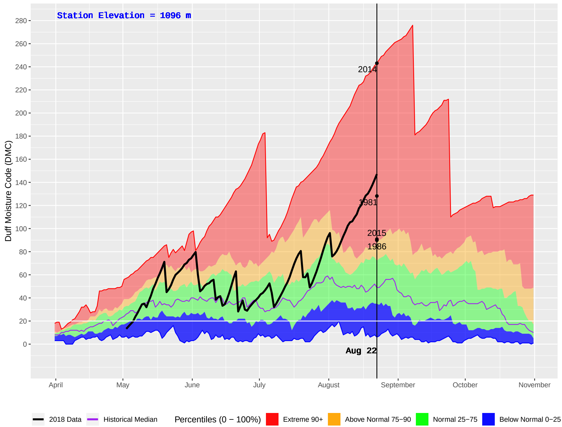
ANAHIM LAKE HUB (213) : Historical (1981–2016) and Current (2018) Daily Duff Moisture Code (DMC)
